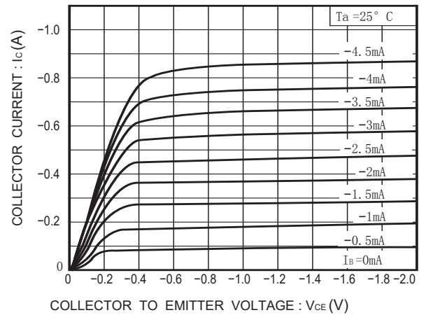
Fig.2 Grounded emitter output characteristics
