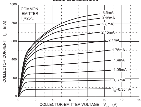
Static Characteristic
