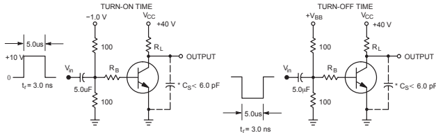
Figure 1. Switching Time Test Circuits
